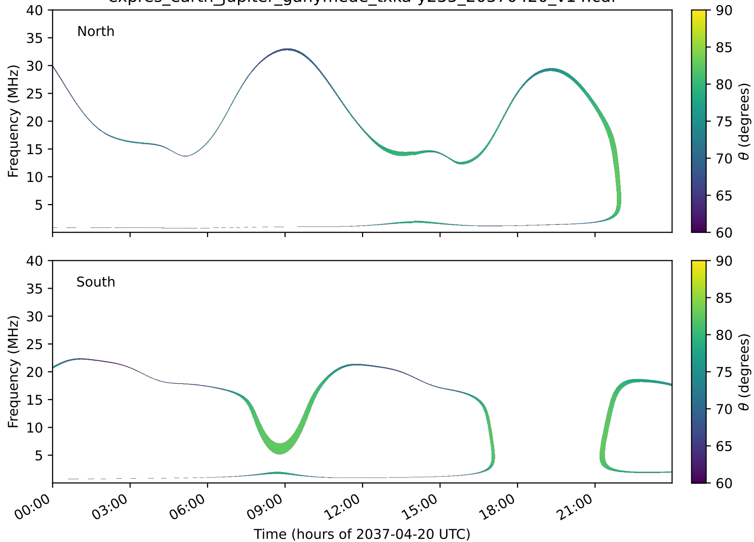
expres_earth_jupiter_ganymede_txka-y235_20370420_v14.cdf
