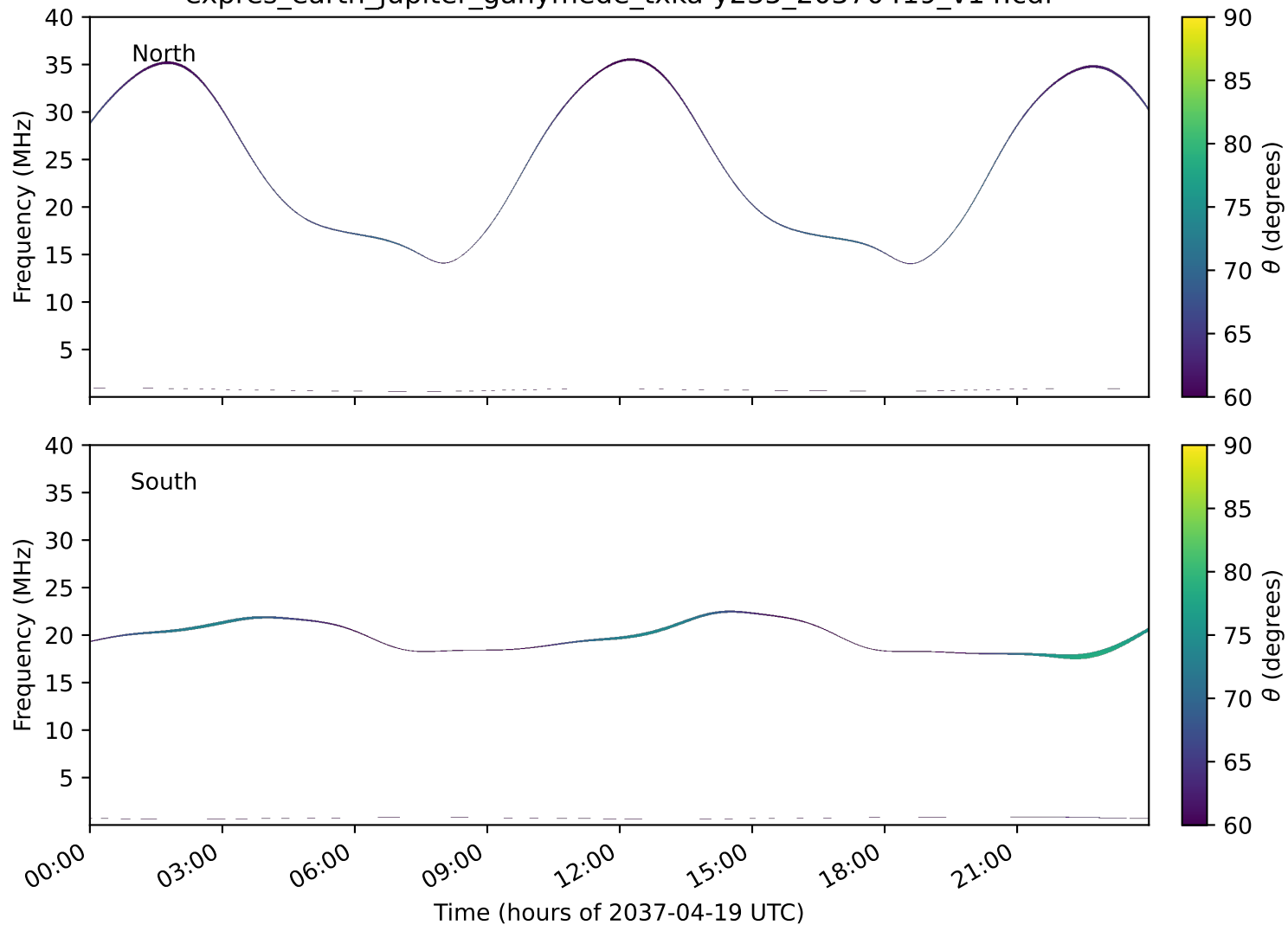
expres_earth_jupiter_ganymede_txka-y235_20370419_v14.cdf
