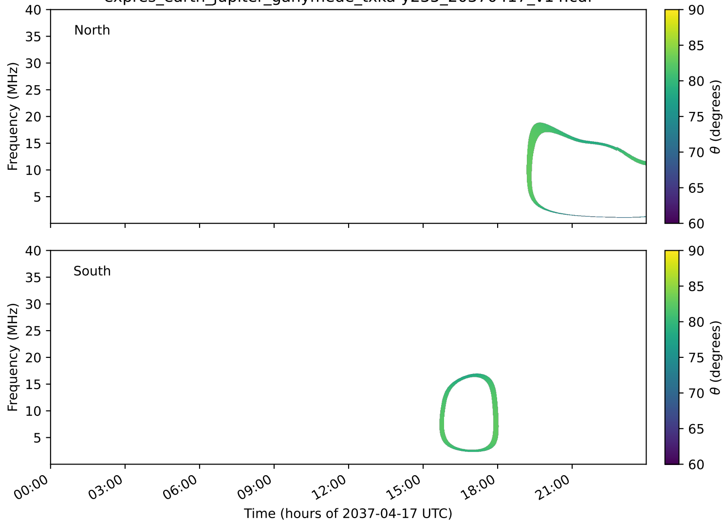
expres_earth_jupiter_ganymede_txka-y235_20370417_v14.cdf
