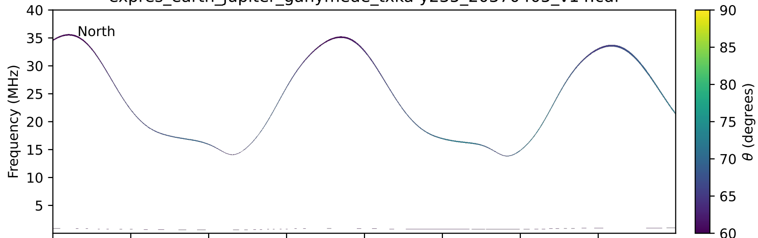
expres_earth_jupiter_ganymede_txka-y235_20370405_v14.cdf
