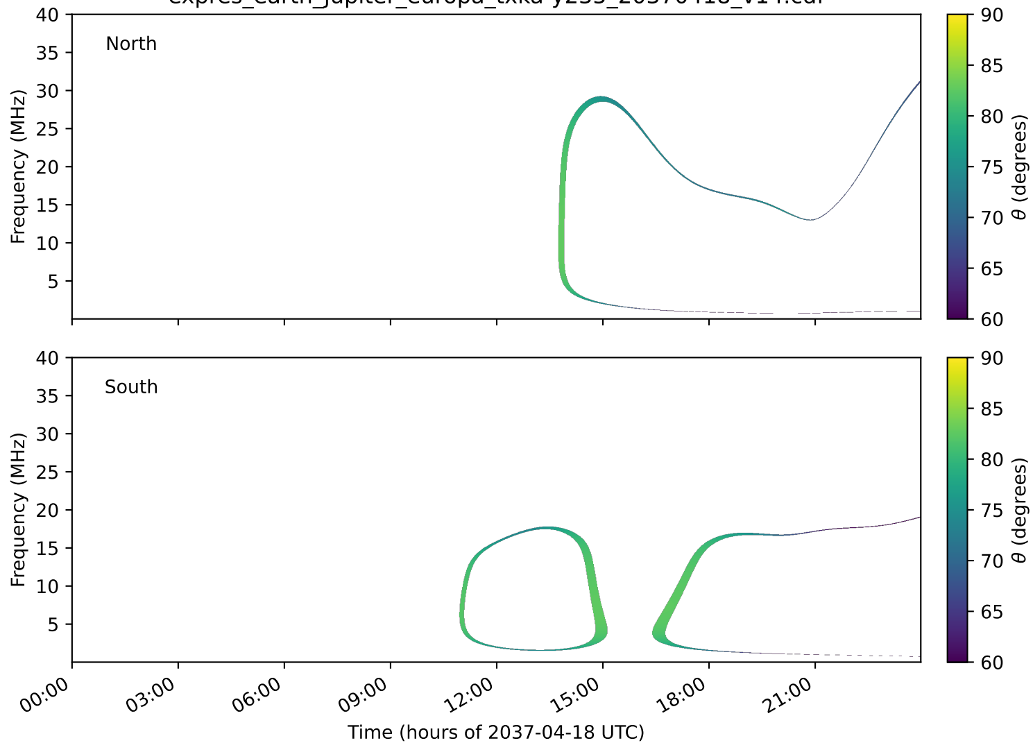
expres_earth_jupiter_europa_txka-y235_20370418_v14.cdf
