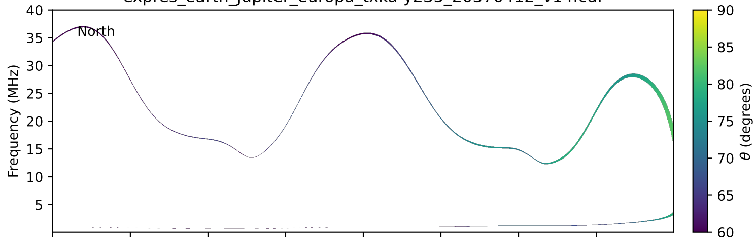
expres_earth_jupiter_europa_txka-y235_20370412_v14.cdf
