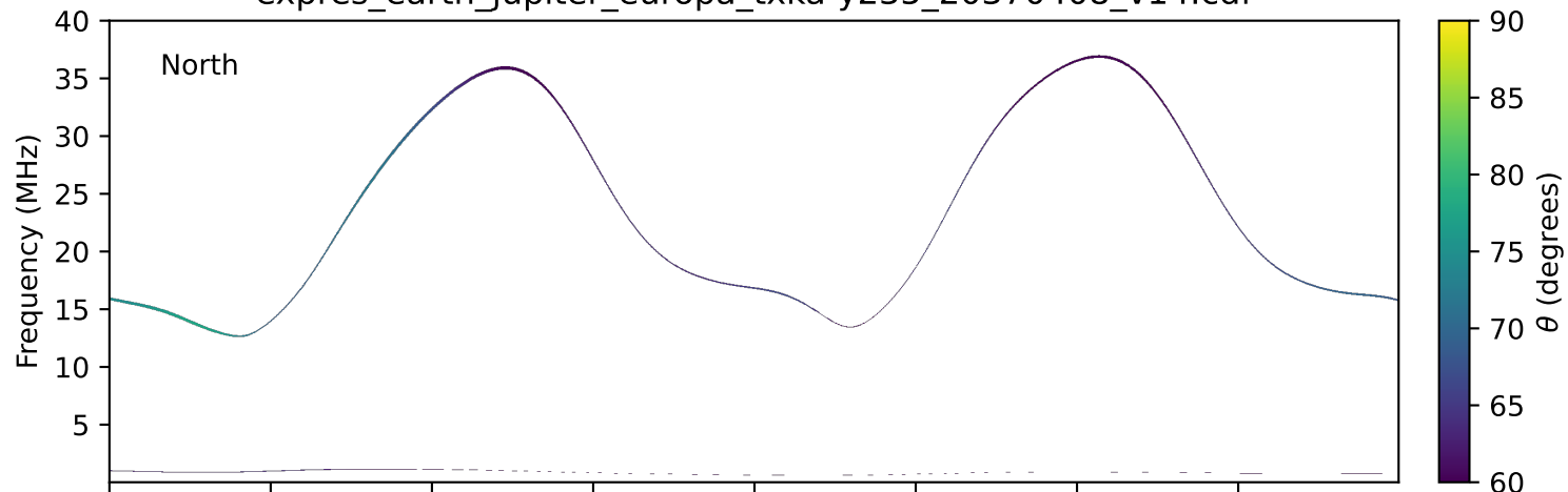
expres_earth_jupiter_europa_txka-y235_20370408_v14.cdf
