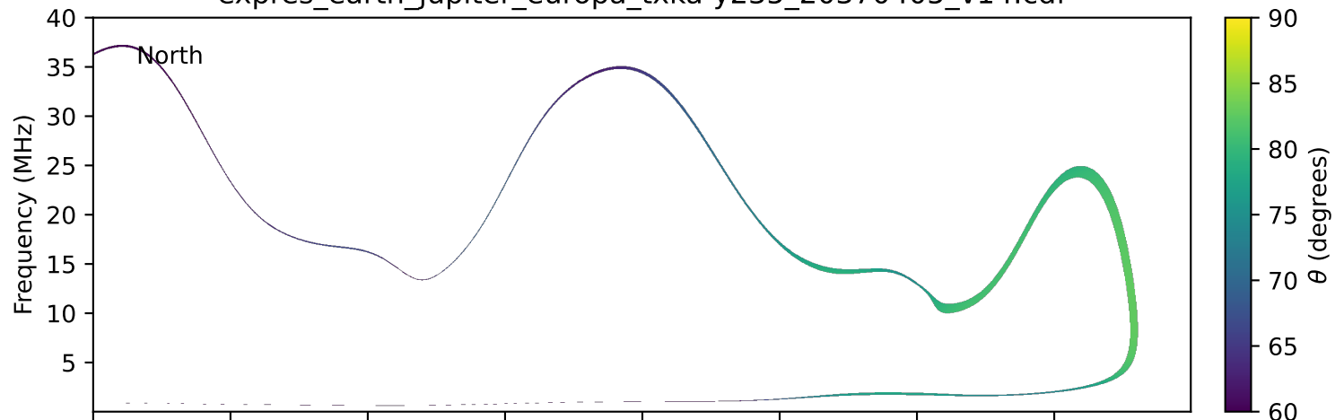
expres_earth_jupiter_europa_txka-y235_20370405_v14.cdf
