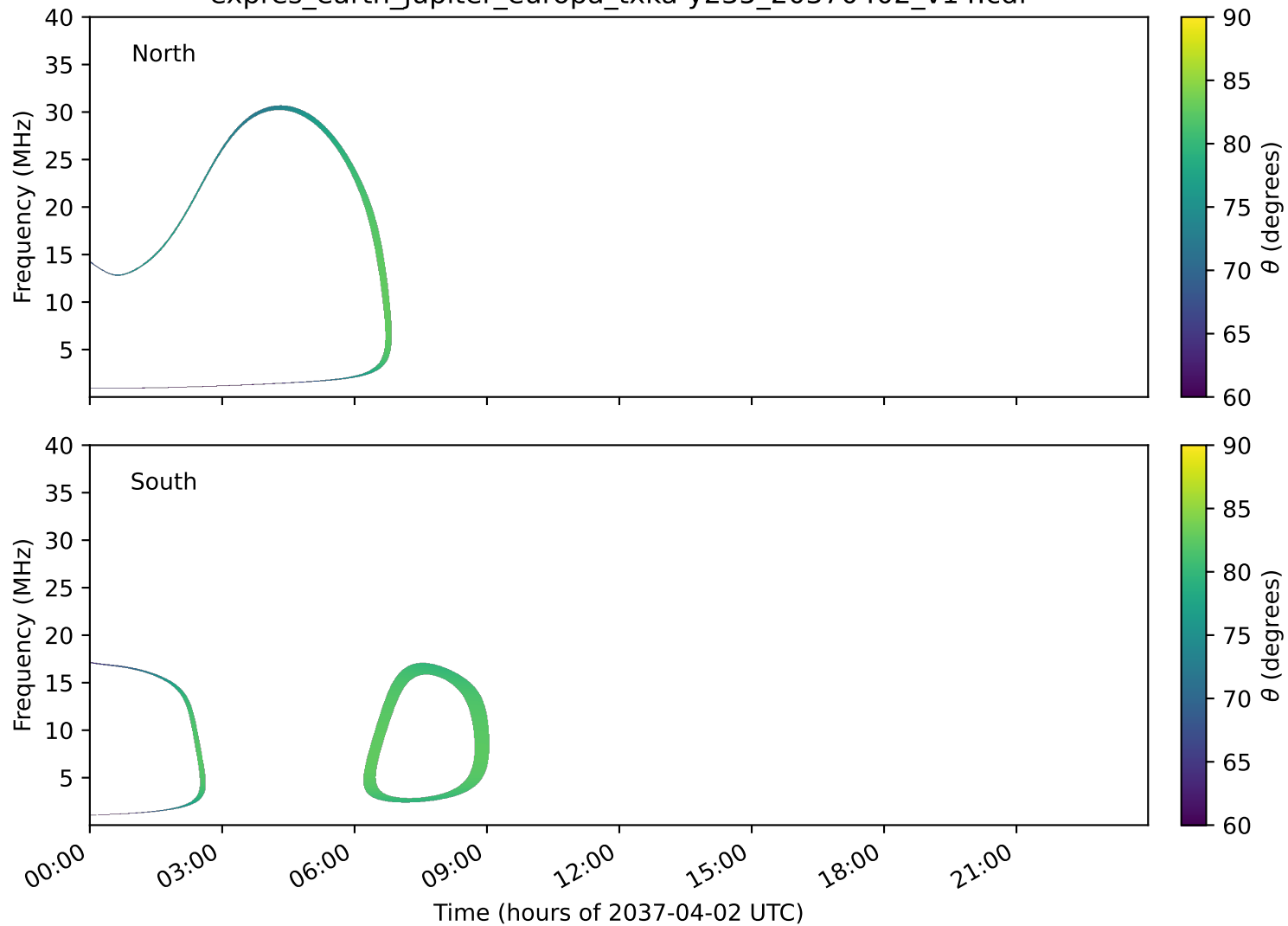
expres_earth_jupiter_europa_txka-y235_20370402_v14.cdf
