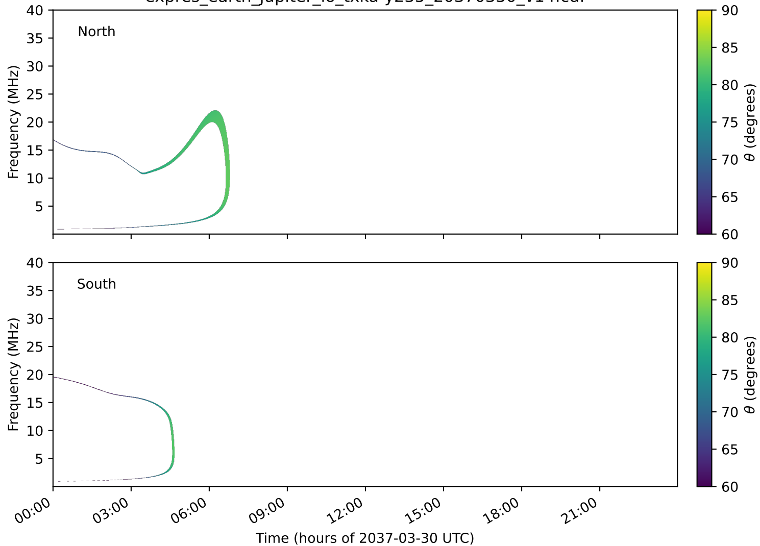
expres_earth_jupiter_io_txka-y235_20370330_v14.cdf
