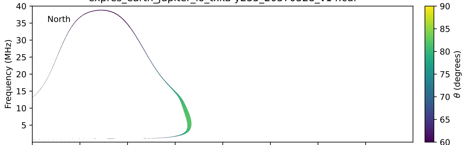
expres_earth_jupiter_io_txka-y235_20370328_v14.cdf
