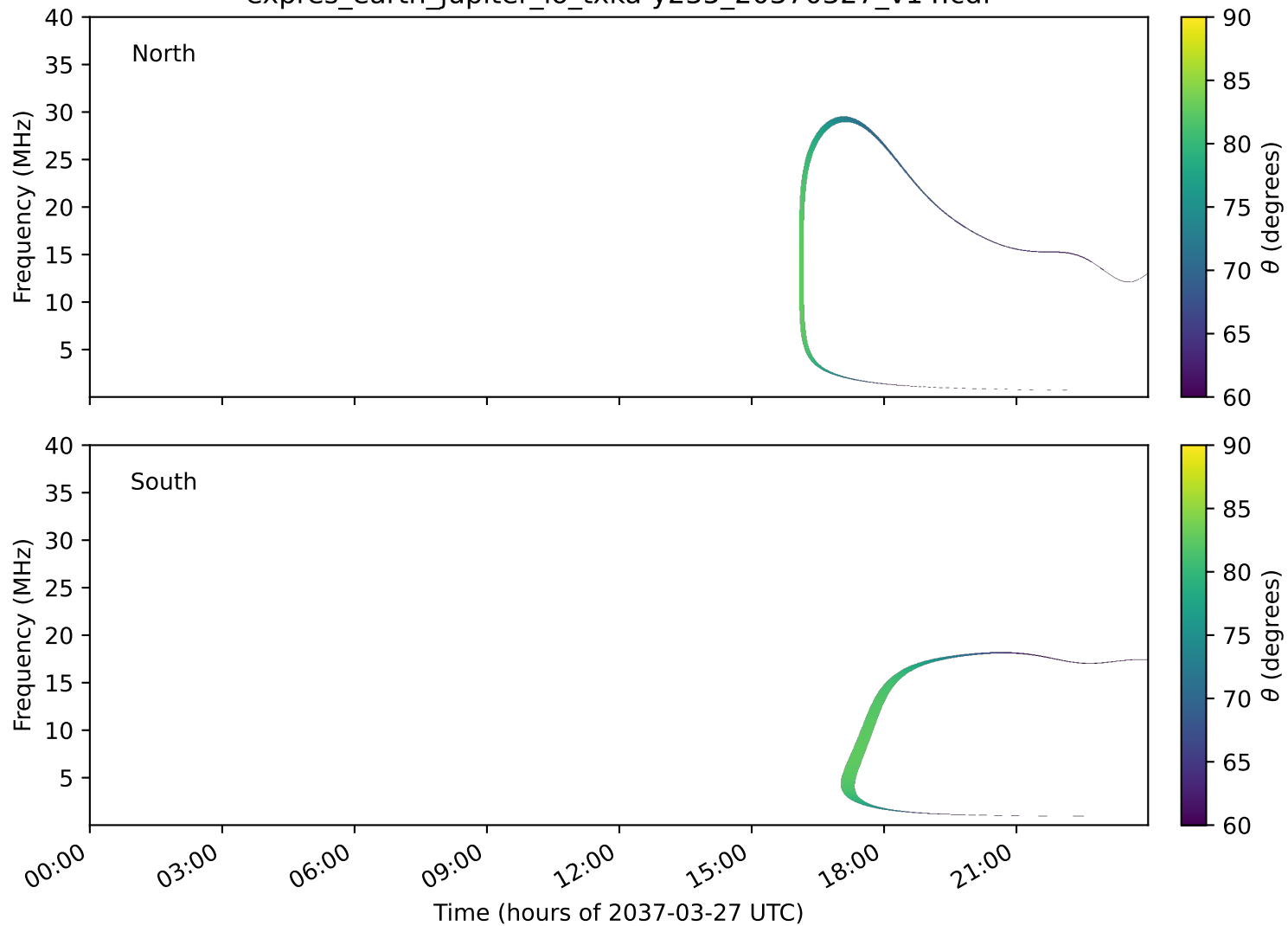
expres_earth_jupiter_io_txka-y235_20370327_v14.cdf
