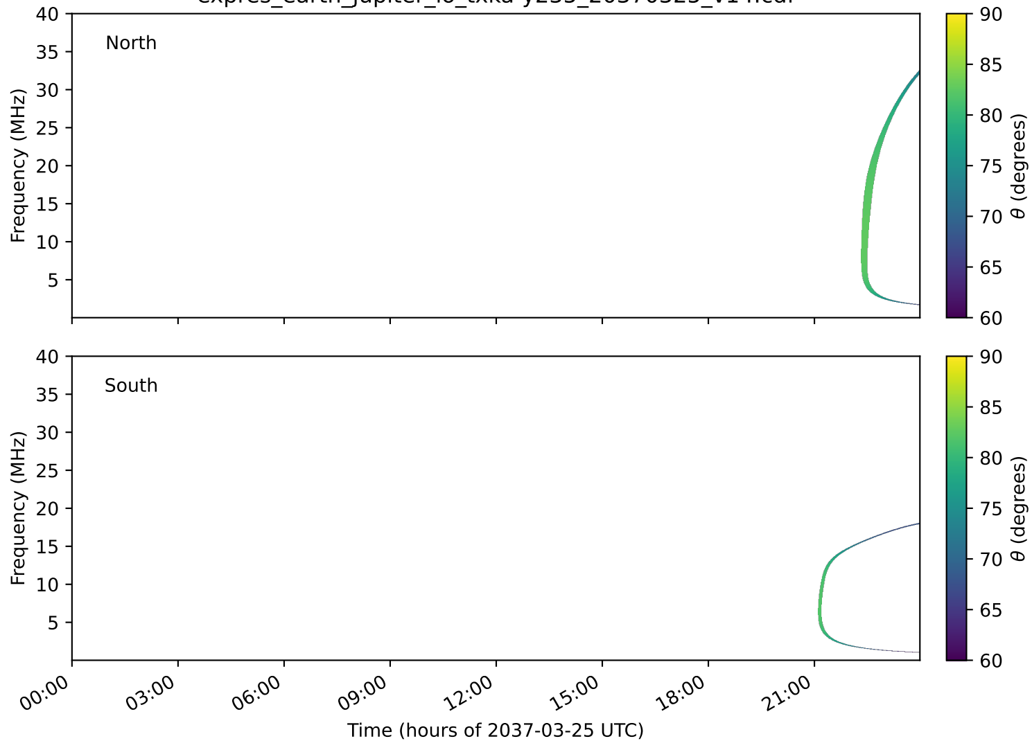
expres_earth_jupiter_io_txka-y235_20370325_v14.cdf
