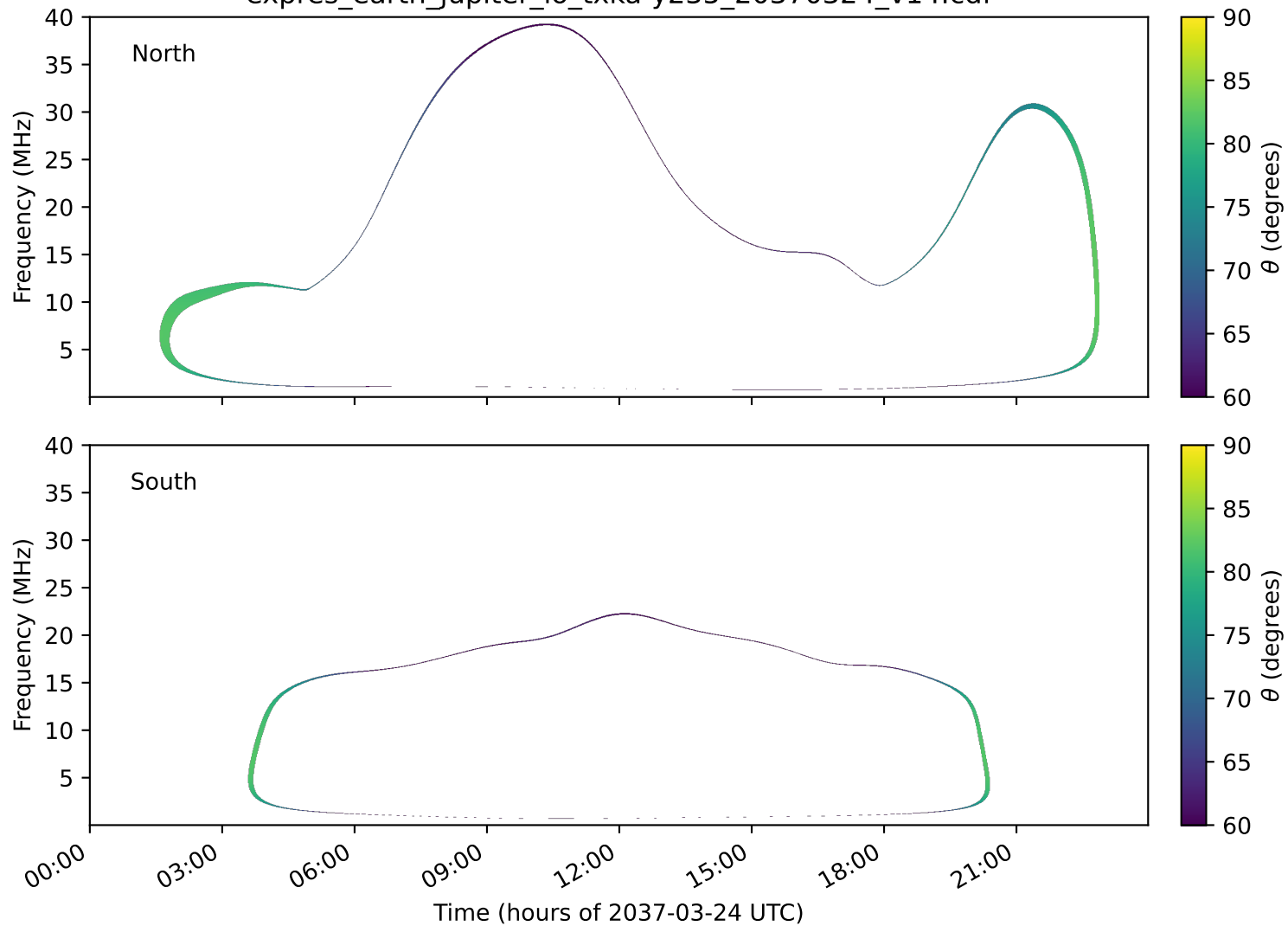
expres_earth_jupiter_io_txka-y235_20370324_v14.cdf
