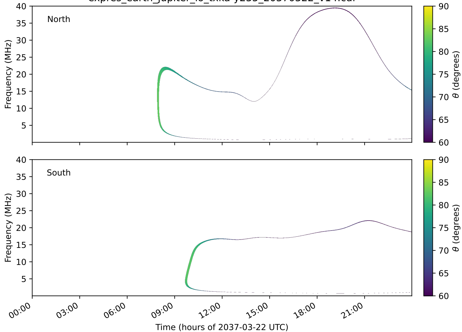
expres_earth_jupiter_io_txka-y235_20370322_v14.cdf
