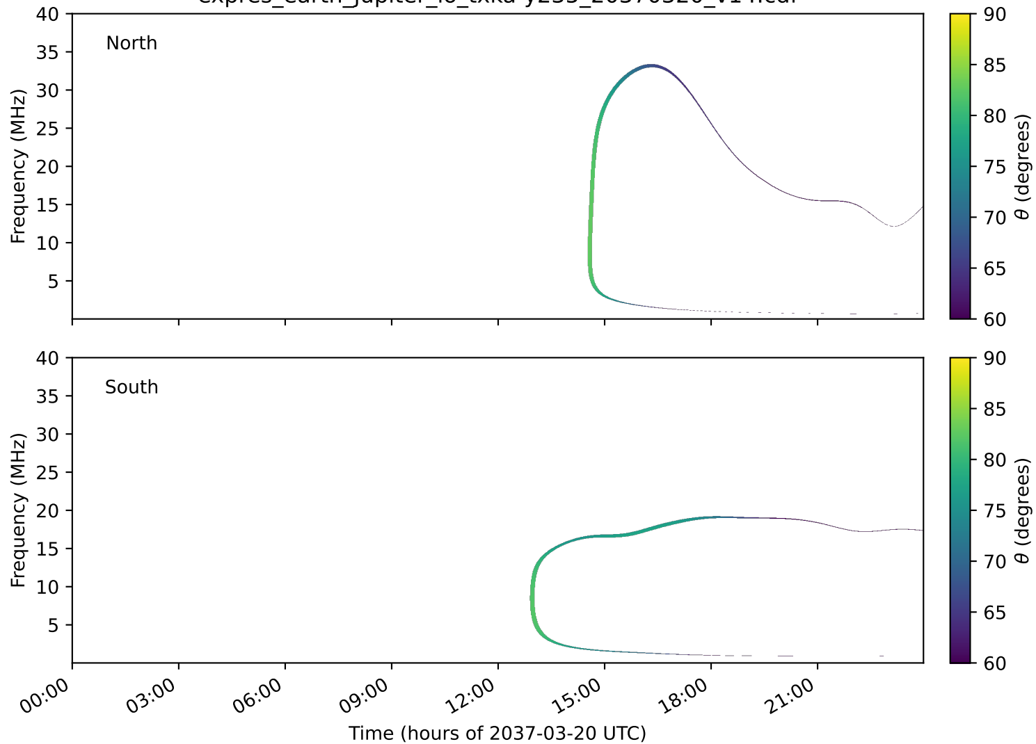
expres_earth_jupiter_io_txka-y235_20370320_v14.cdf
