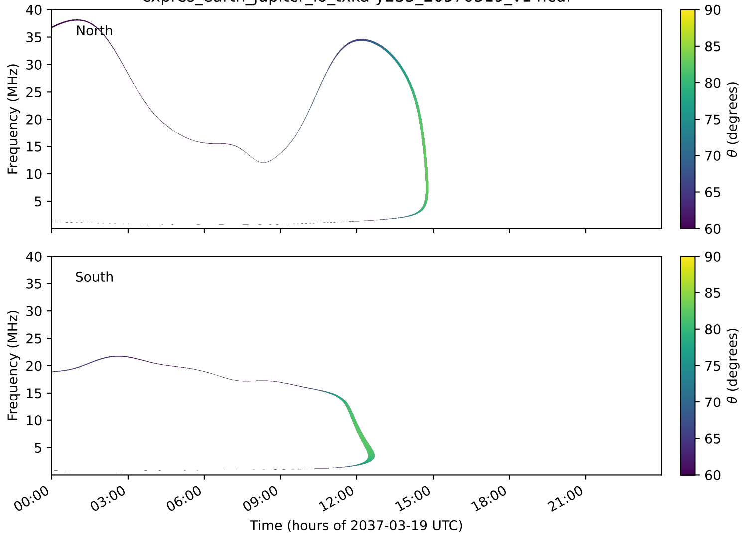
expres_earth_jupiter_io_txka-y235_20370319_v14.cdf
