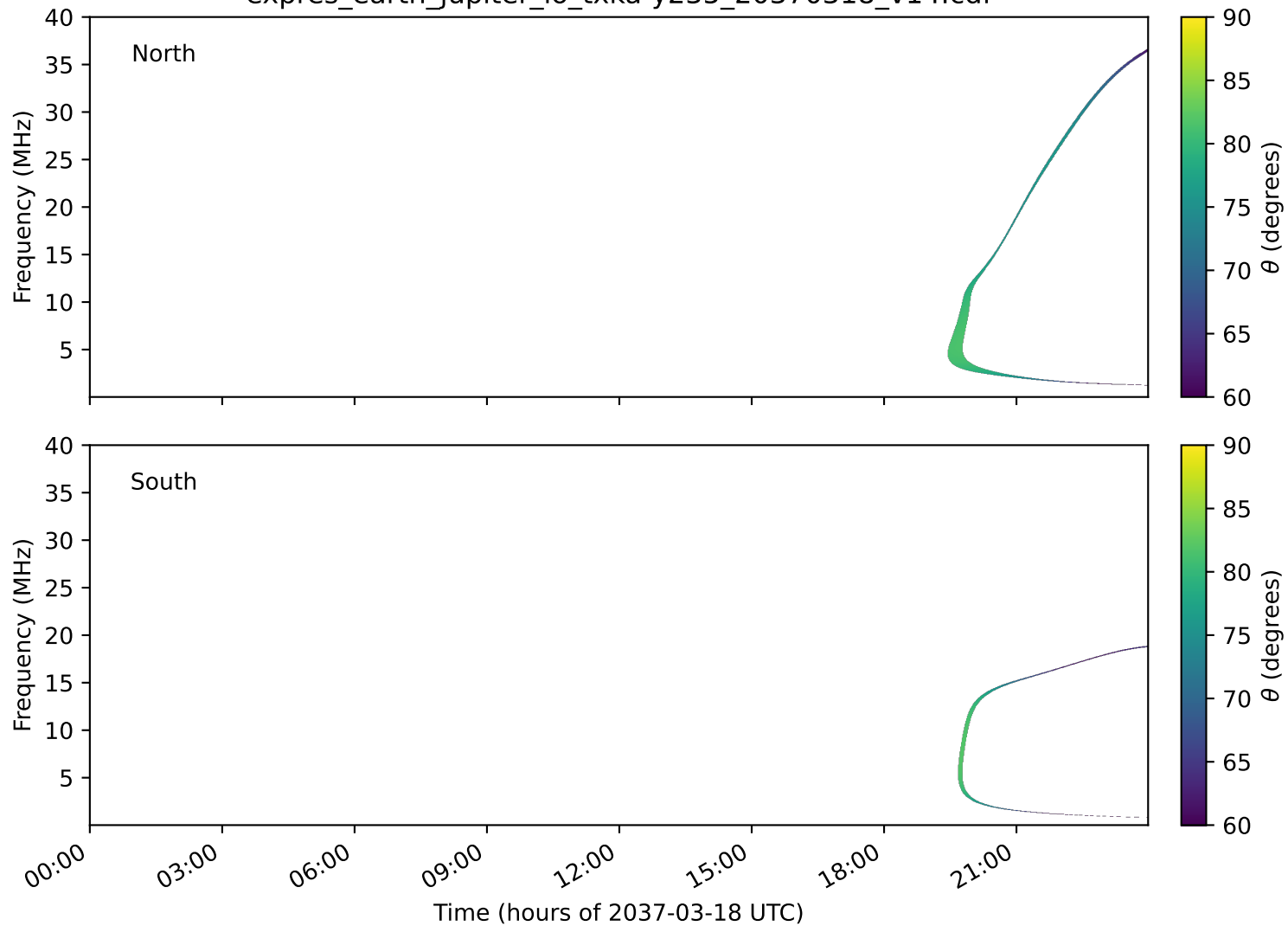
expres_earth_jupiter_io_txka-y235_20370318_v14.cdf
