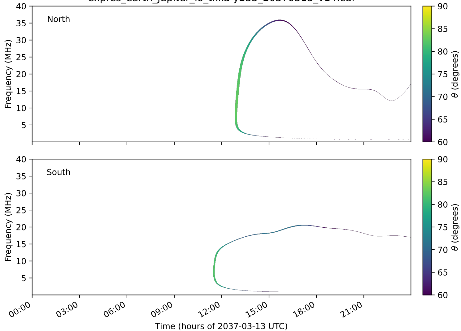
expres_earth_jupiter_io_txka-y235_20370313_v14.cdf
