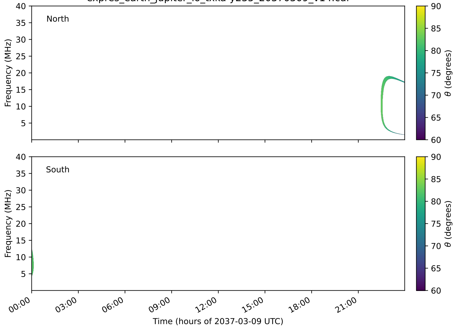
expres_earth_jupiter_io_txka-y235_20370309_v14.cdf
