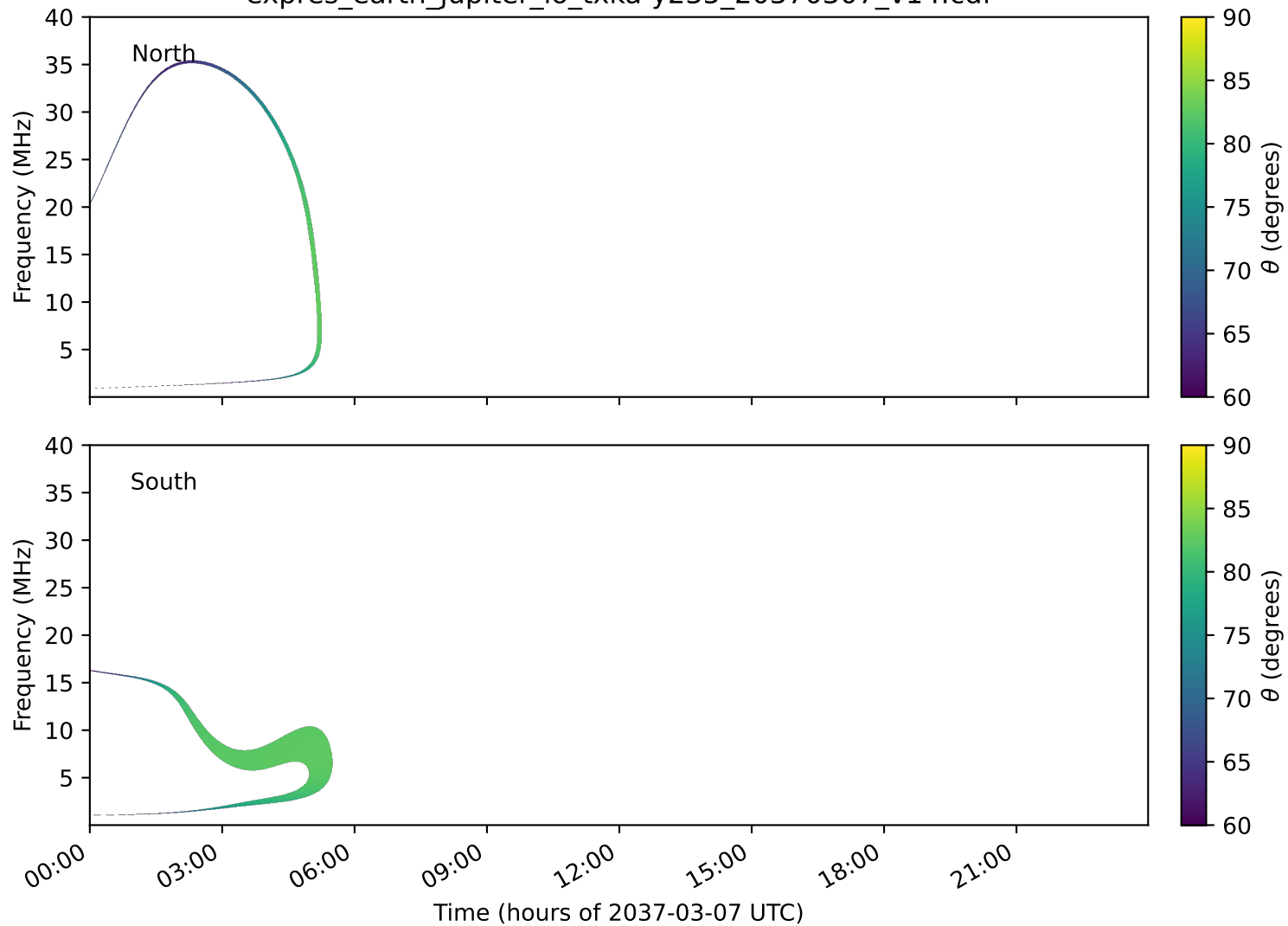
expres_earth_jupiter_io_txka-y235_20370307_v14.cdf
