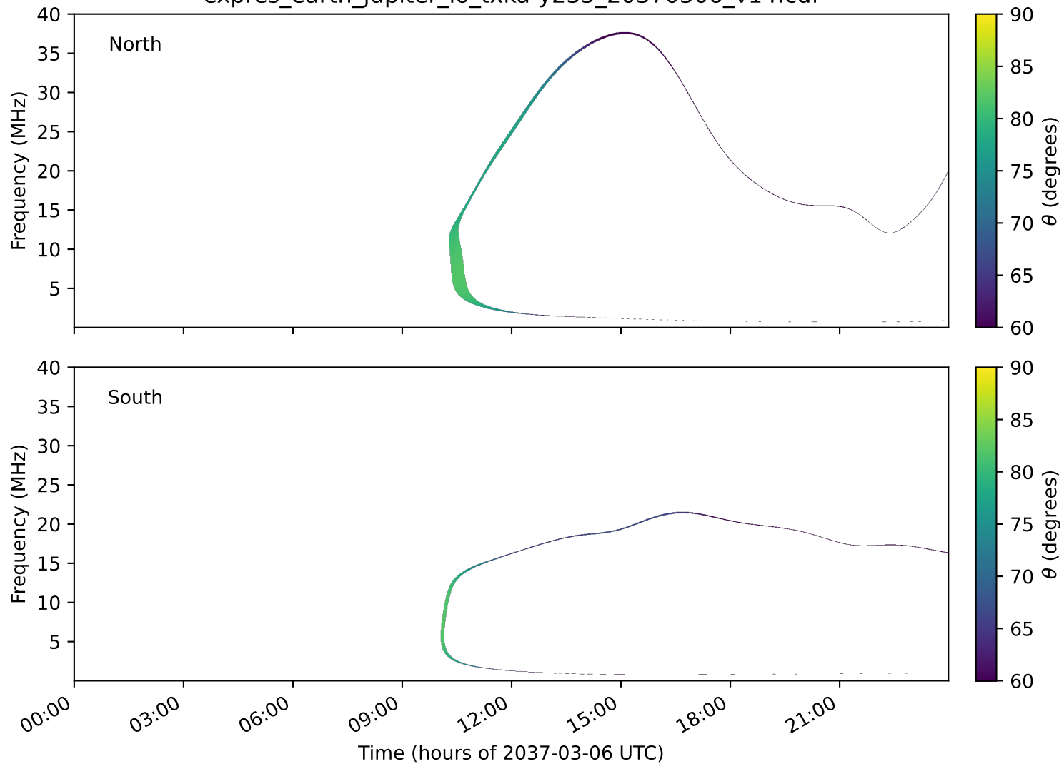
expres_earth_jupiter_io_txka-y235_20370306_v14.cdf
