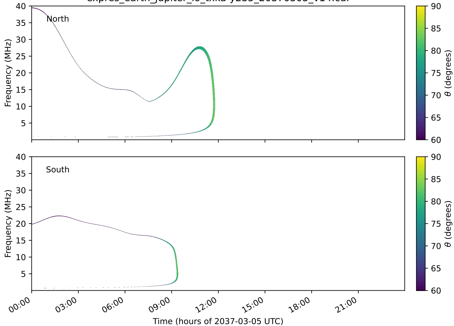
expres_earth_jupiter_io_txka-y235_20370305_v14.cdf
