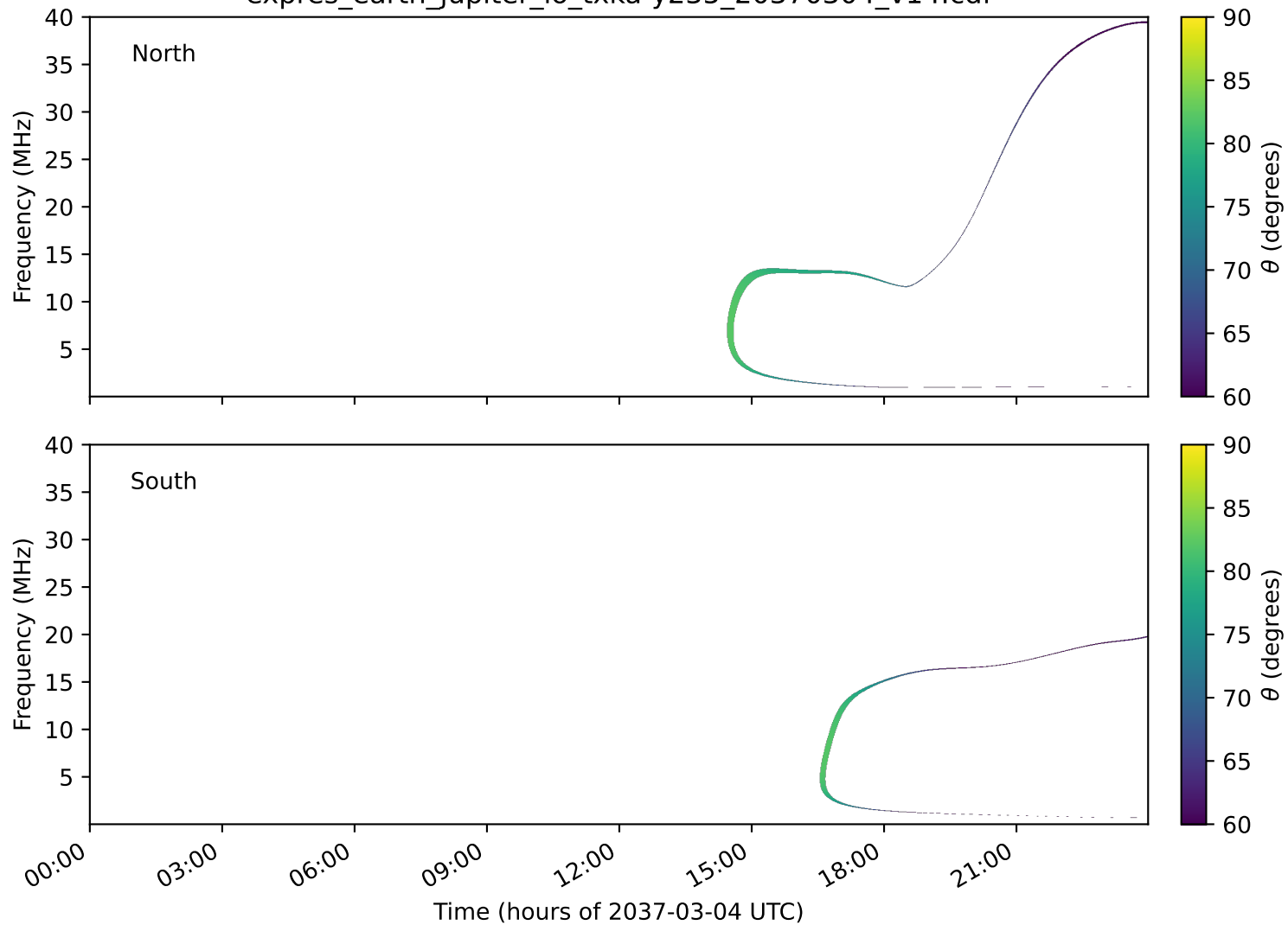
expres_earth_jupiter_io_txka-y235_20370304_v14.cdf
