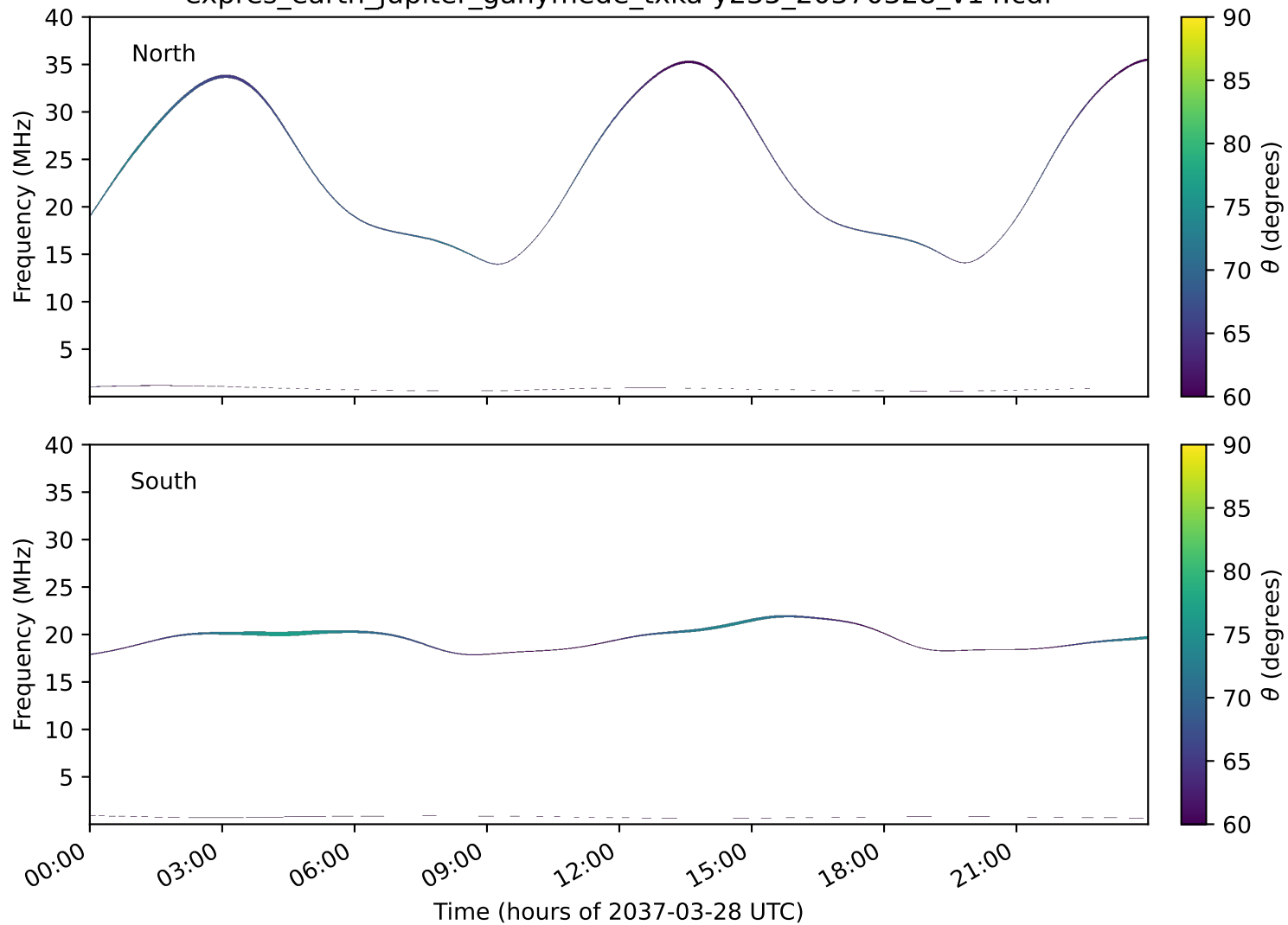
expres_earth_jupiter_ganymede_txka-y235_20370328_v14.cdf
