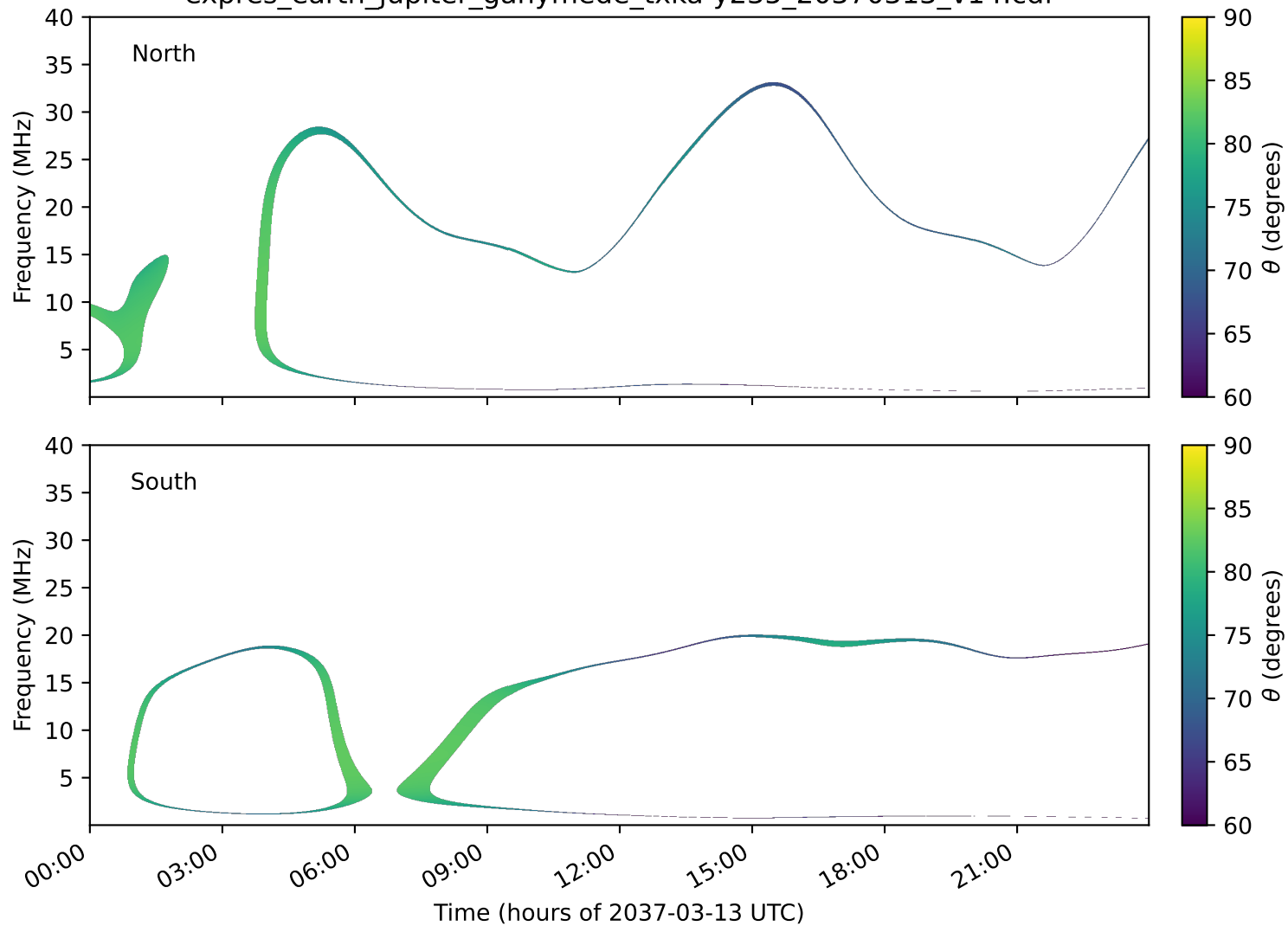
expres_earth_jupiter_ganymede_txka-y235_20370313_v14.cdf
