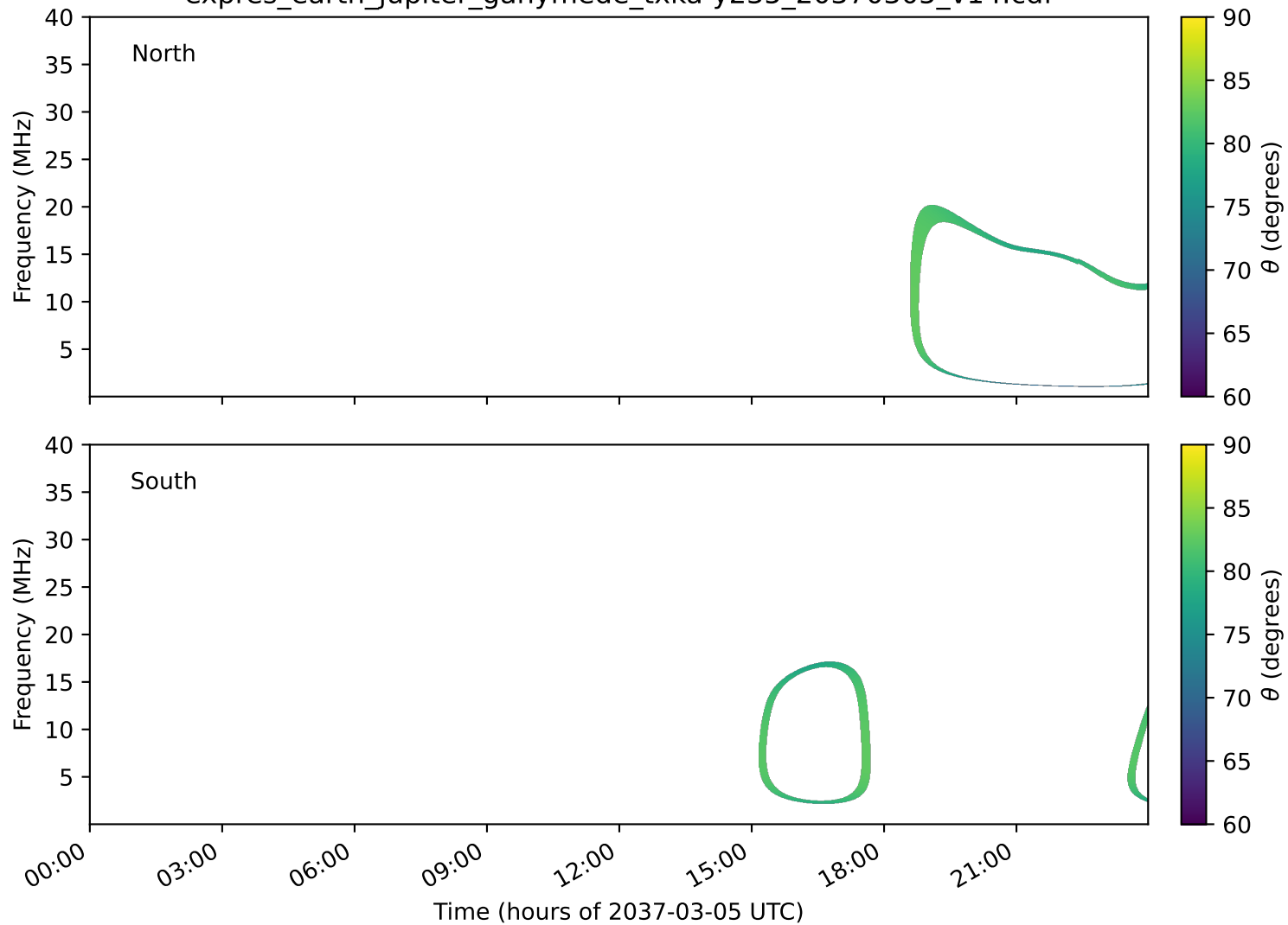
expres_earth_jupiter_ganymede_txka-y235_20370305_v14.cdf
