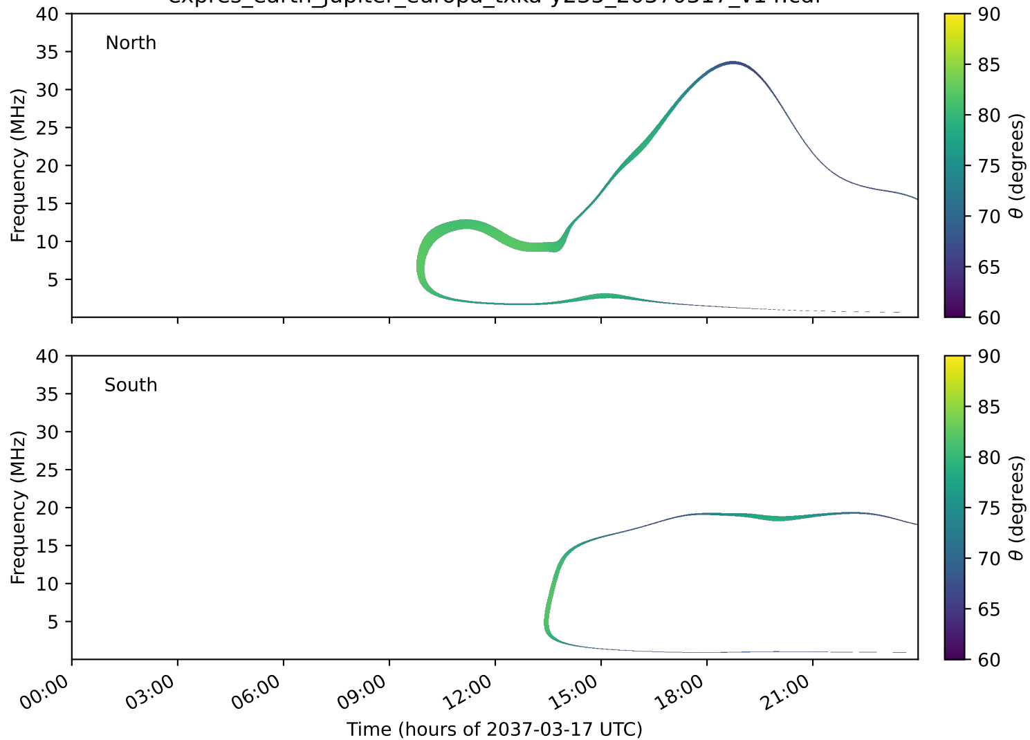
expres_earth_jupiter_europa_txka-y235_20370317_v14.cdf
