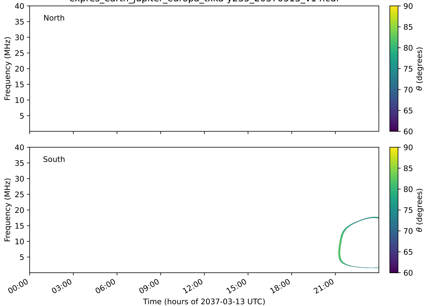
expres_earth_jupiter_europa_txka-y235_20370313_v14.cdf
