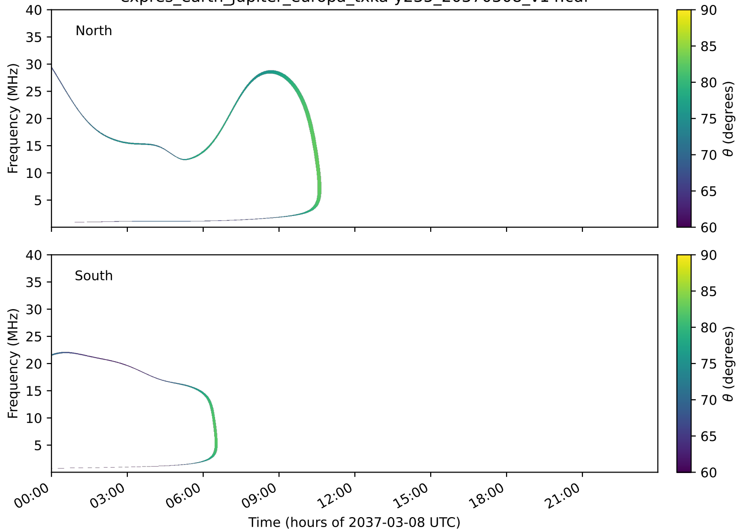
expres_earth_jupiter_europa_txka-y235_20370308_v14.cdf
