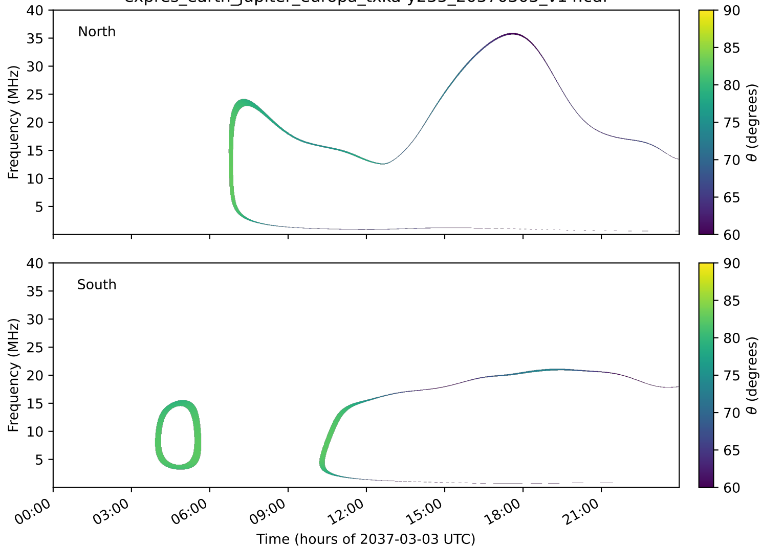
expres_earth_jupiter_europa_txka-y235_20370303_v14.cdf
