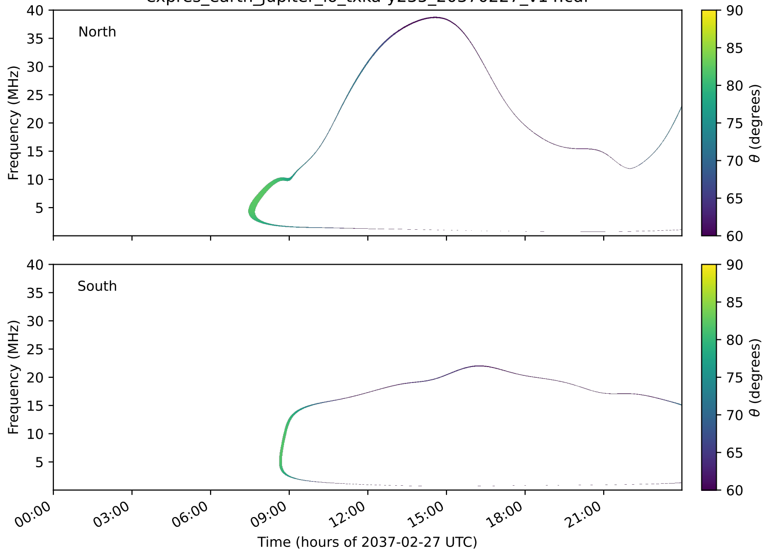
expres_earth_jupiter_io_txka-y235_20370227_v14.cdf
