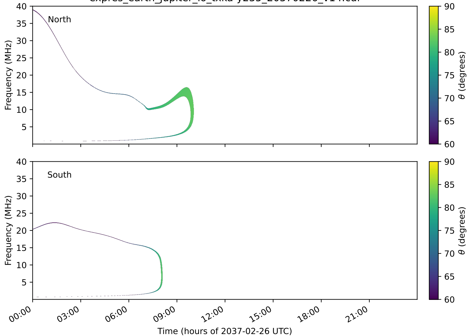
expres_earth_jupiter_io_txka-y235_20370226_v14.cdf
