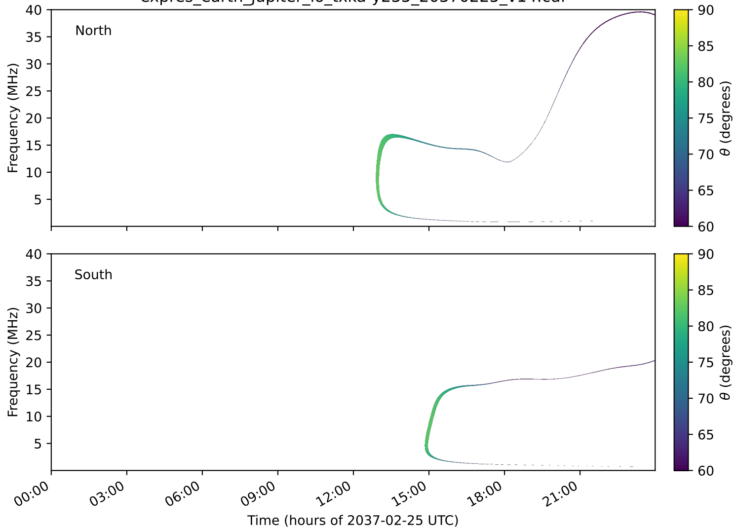
expres_earth_jupiter_io_txka-y235_20370225_v14.cdf
