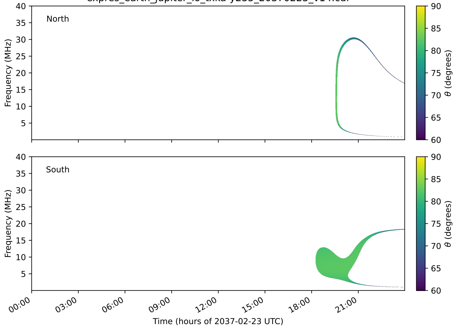
expres_earth_jupiter_io_txka-y235_20370223_v14.cdf
