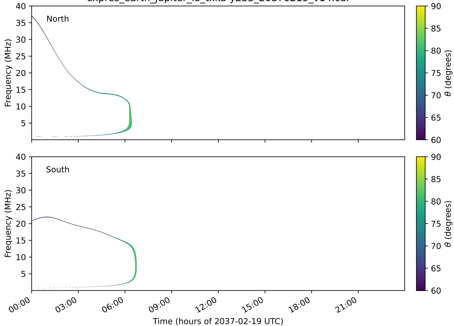
expres_earth_jupiter_io_txka-y235_20370219_v14.cdf
