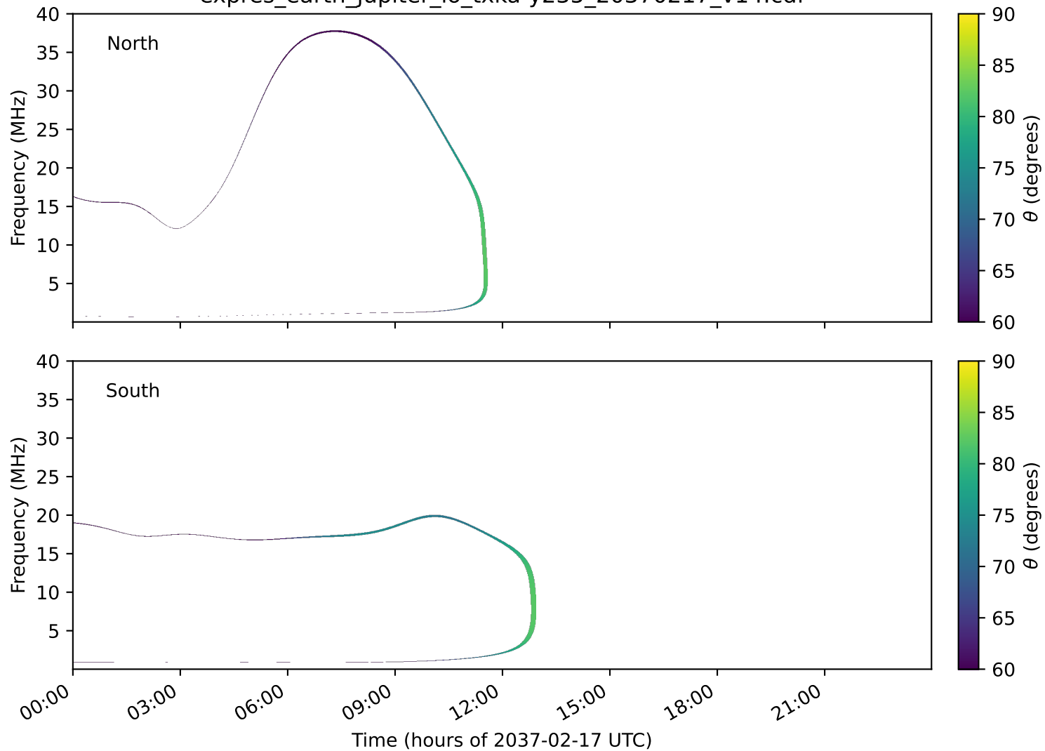
expres_earth_jupiter_io_txka-y235_20370217_v14.cdf
