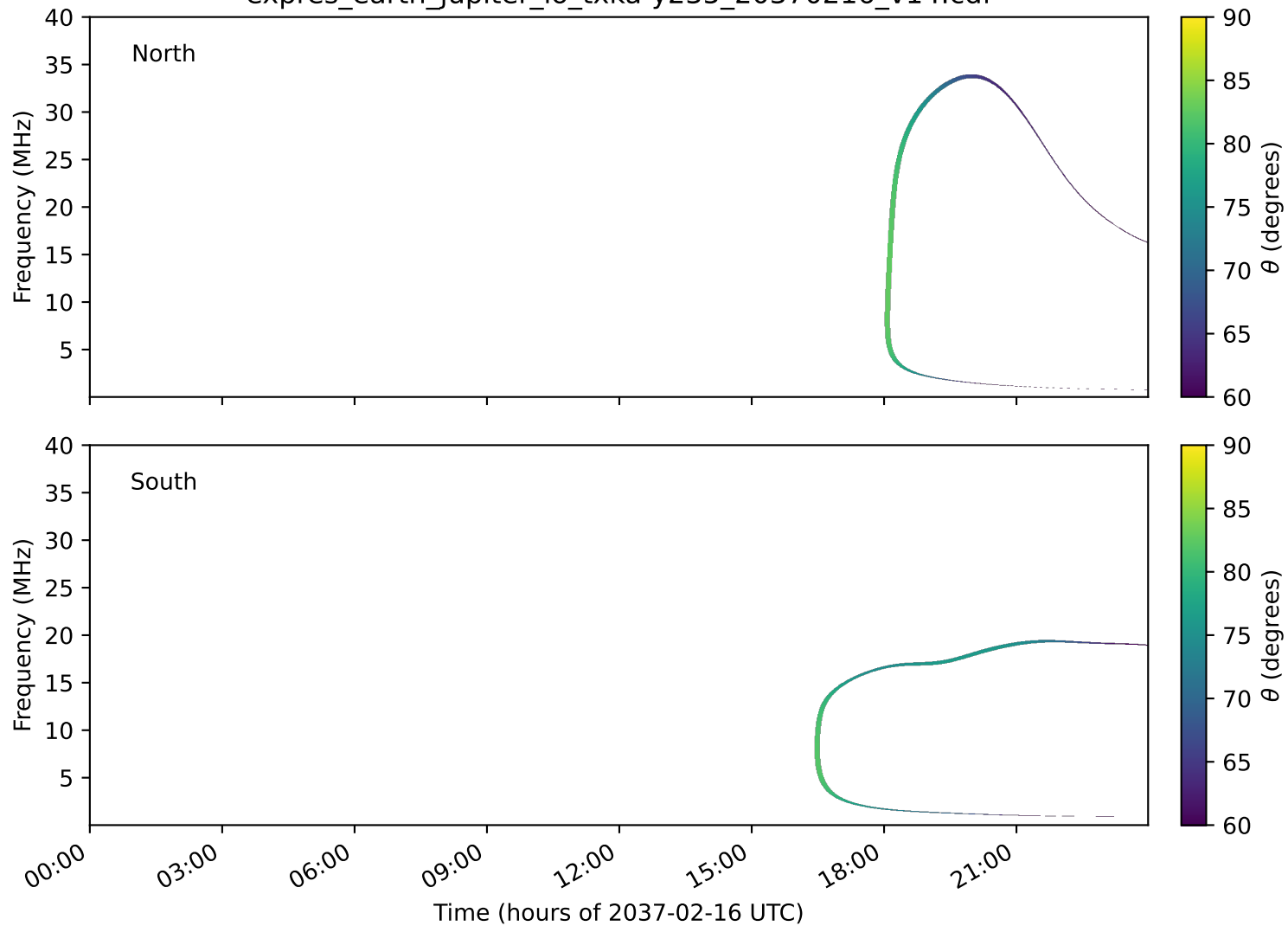
expres_earth_jupiter_io_txka-y235_20370216_v14.cdf
