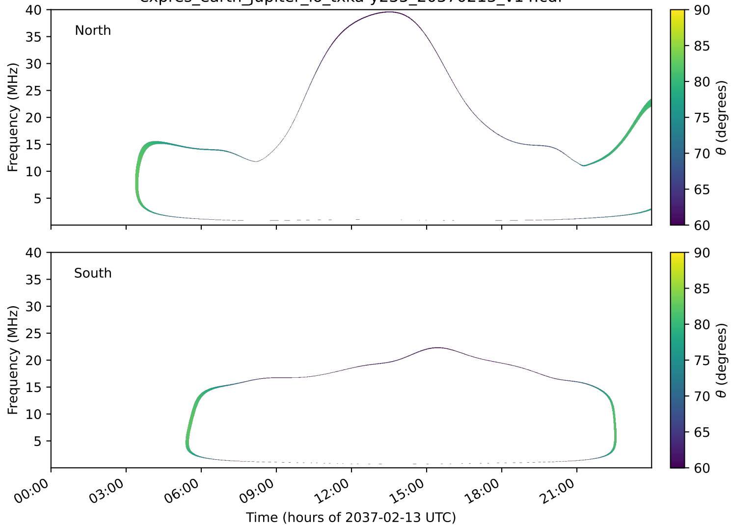
expres_earth_jupiter_io_txka-y235_20370213_v14.cdf
