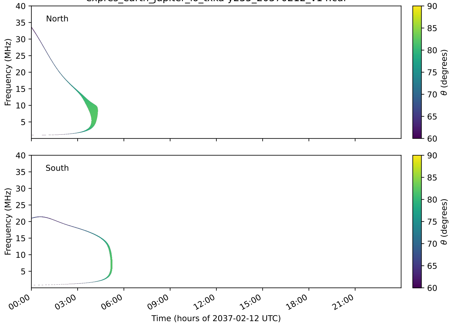
expres_earth_jupiter_io_txka-y235_20370212_v14.cdf
