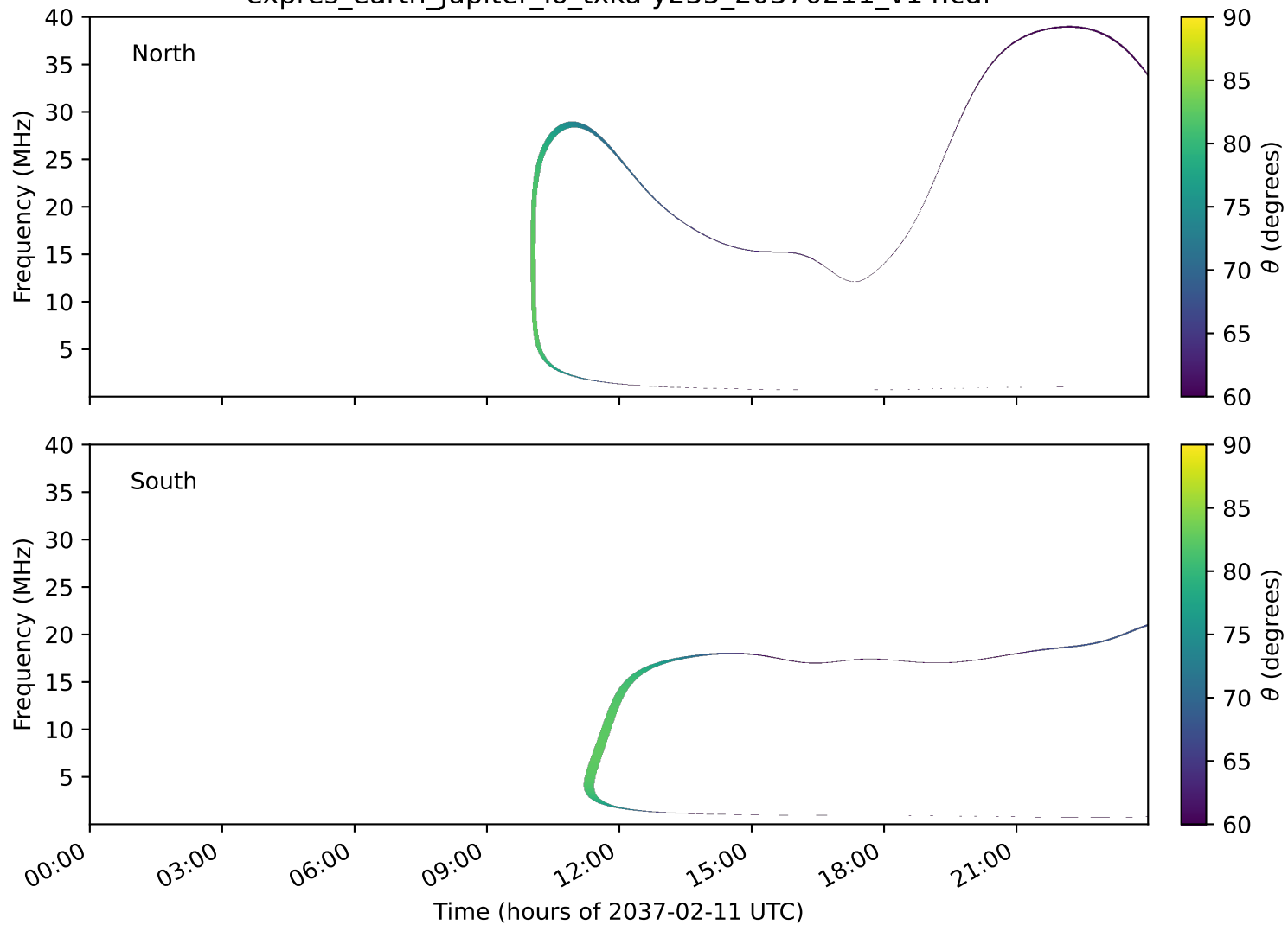
expres_earth_jupiter_io_txka-y235_20370211_v14.cdf
