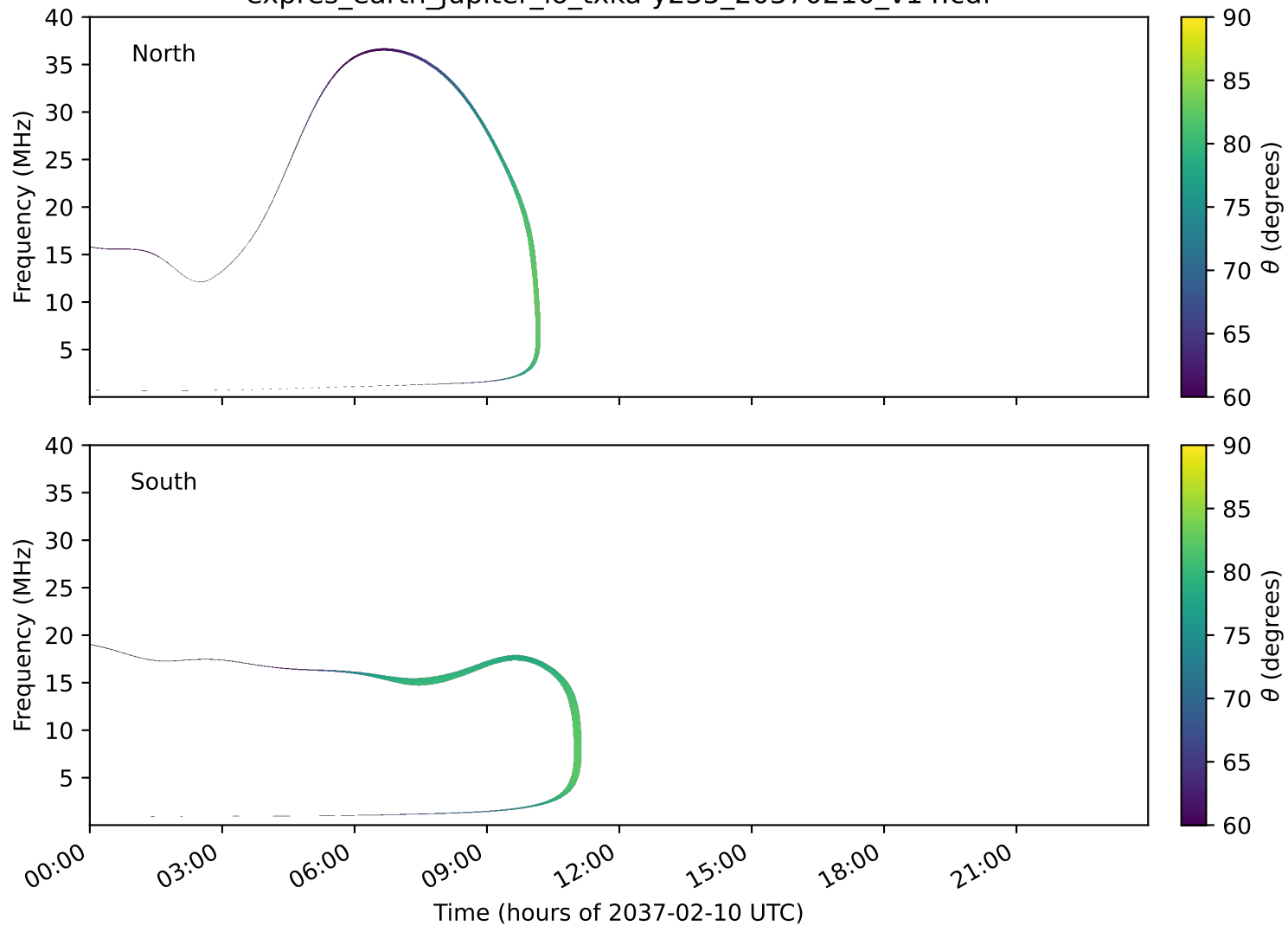
expres_earth_jupiter_io_txka-y235_20370210_v14.cdf
