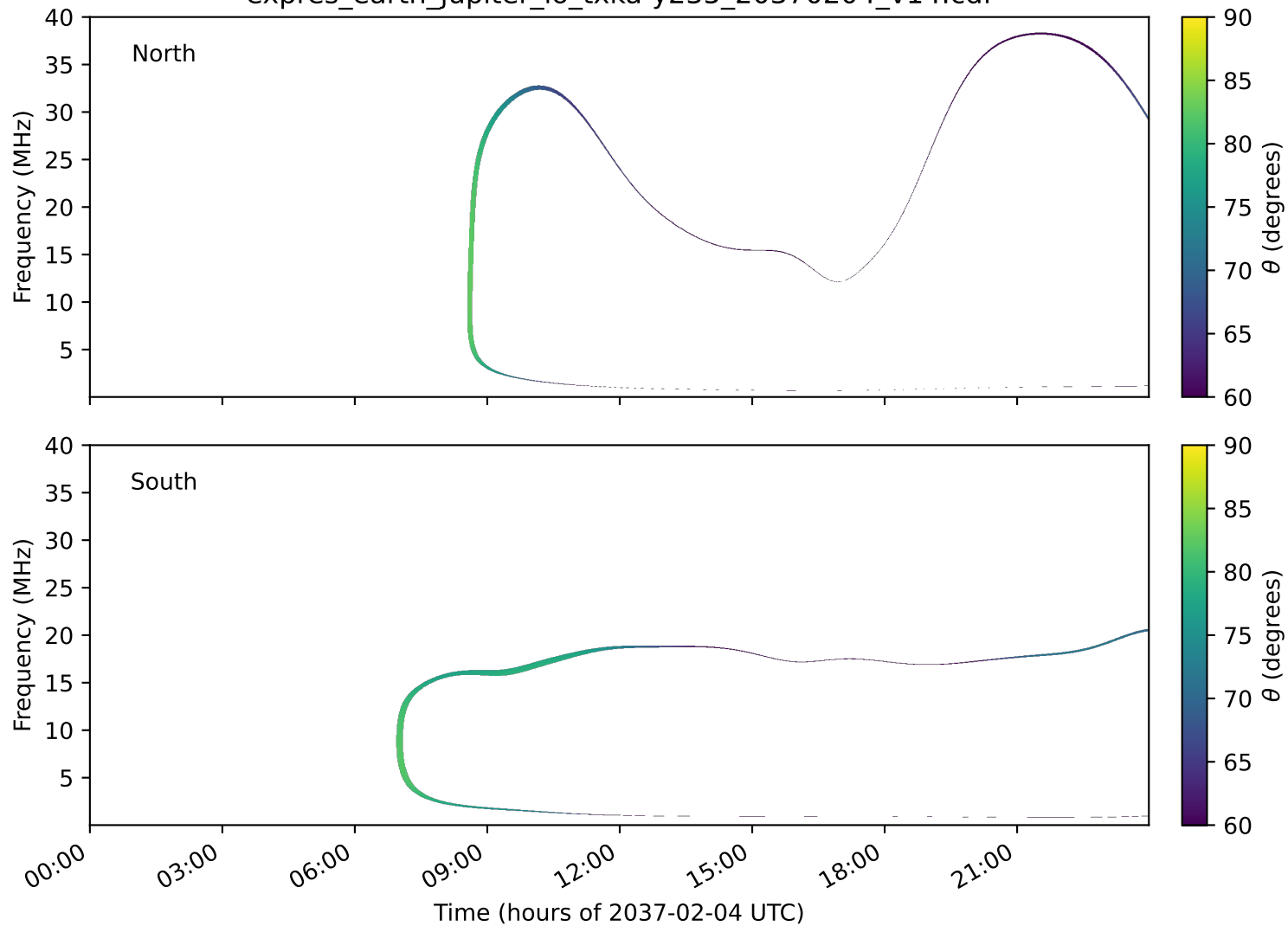
expres_earth_jupiter_io_txka-y235_20370204_v14.cdf
