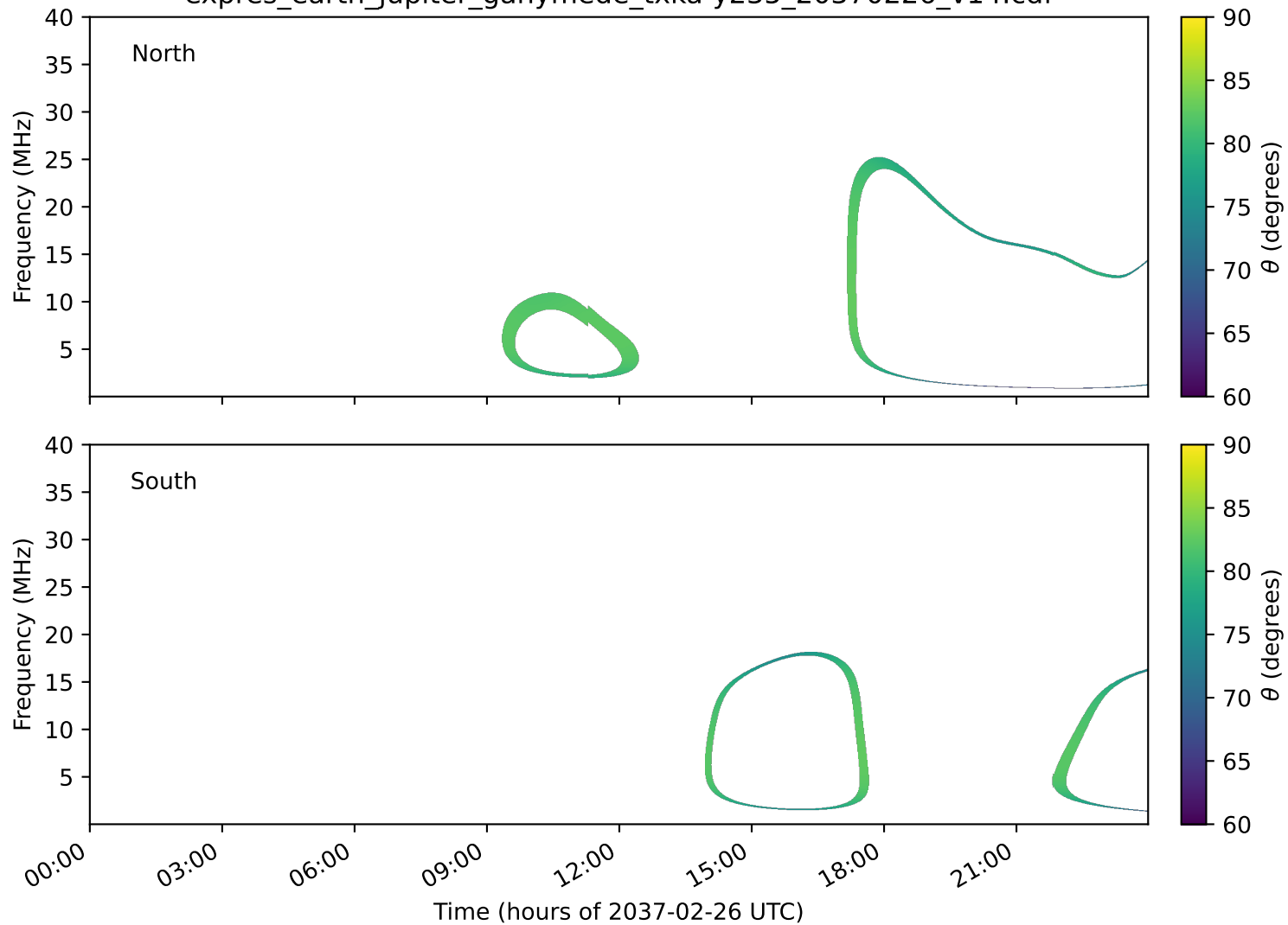
expres_earth_jupiter_ganymede_txka-y235_20370226_v14.cdf
