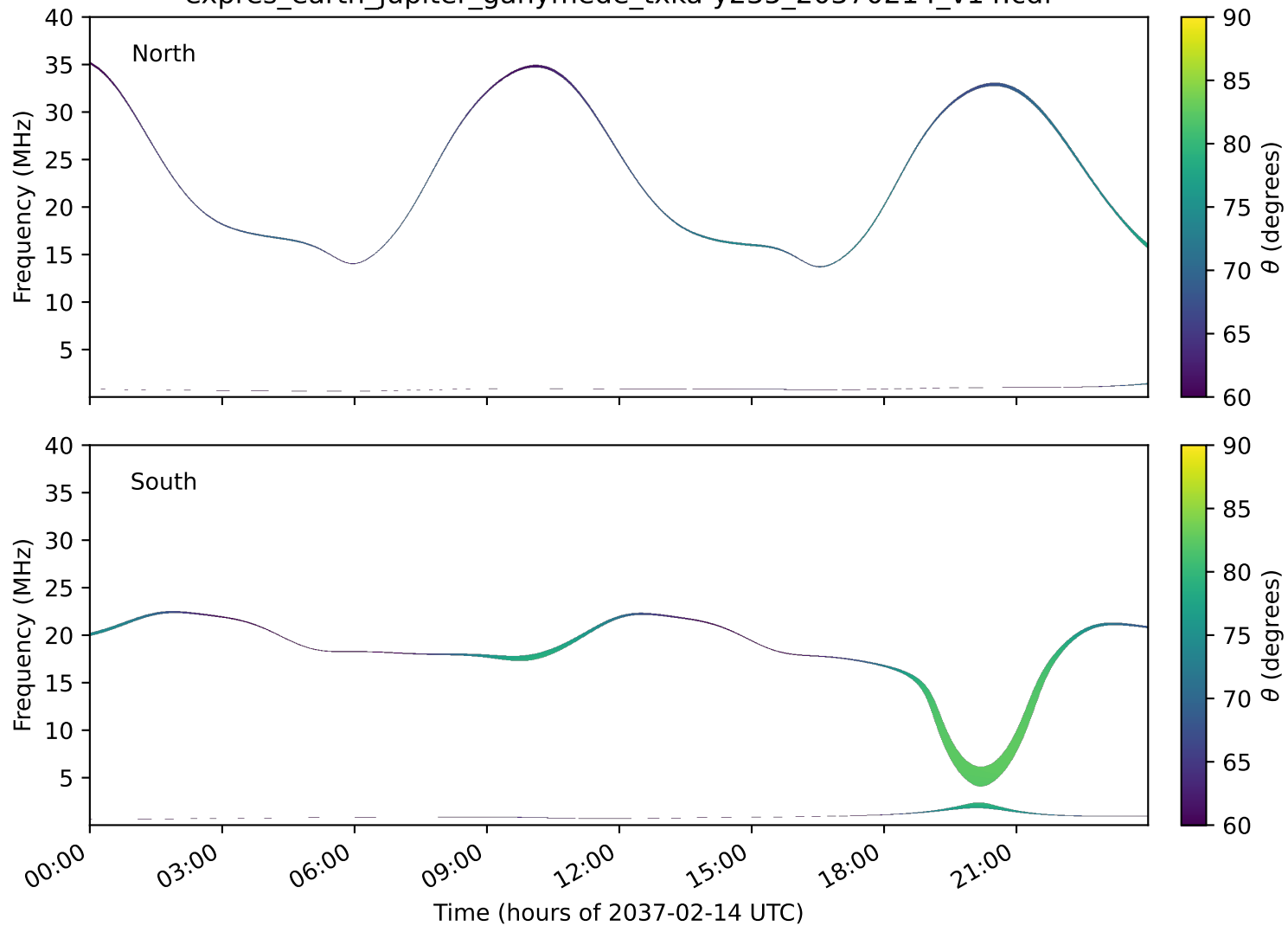
expres_earth_jupiter_ganymede_txka-y235_20370214_v14.cdf
