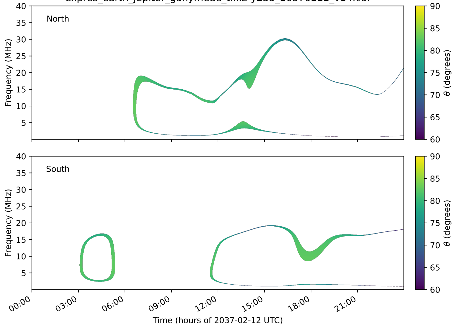
expres_earth_jupiter_ganymede_txka-y235_20370212_v14.cdf
