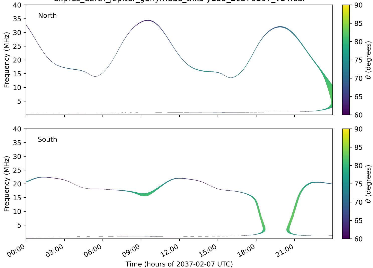
expres_earth_jupiter_ganymede_txka-y235_20370207_v14.cdf
