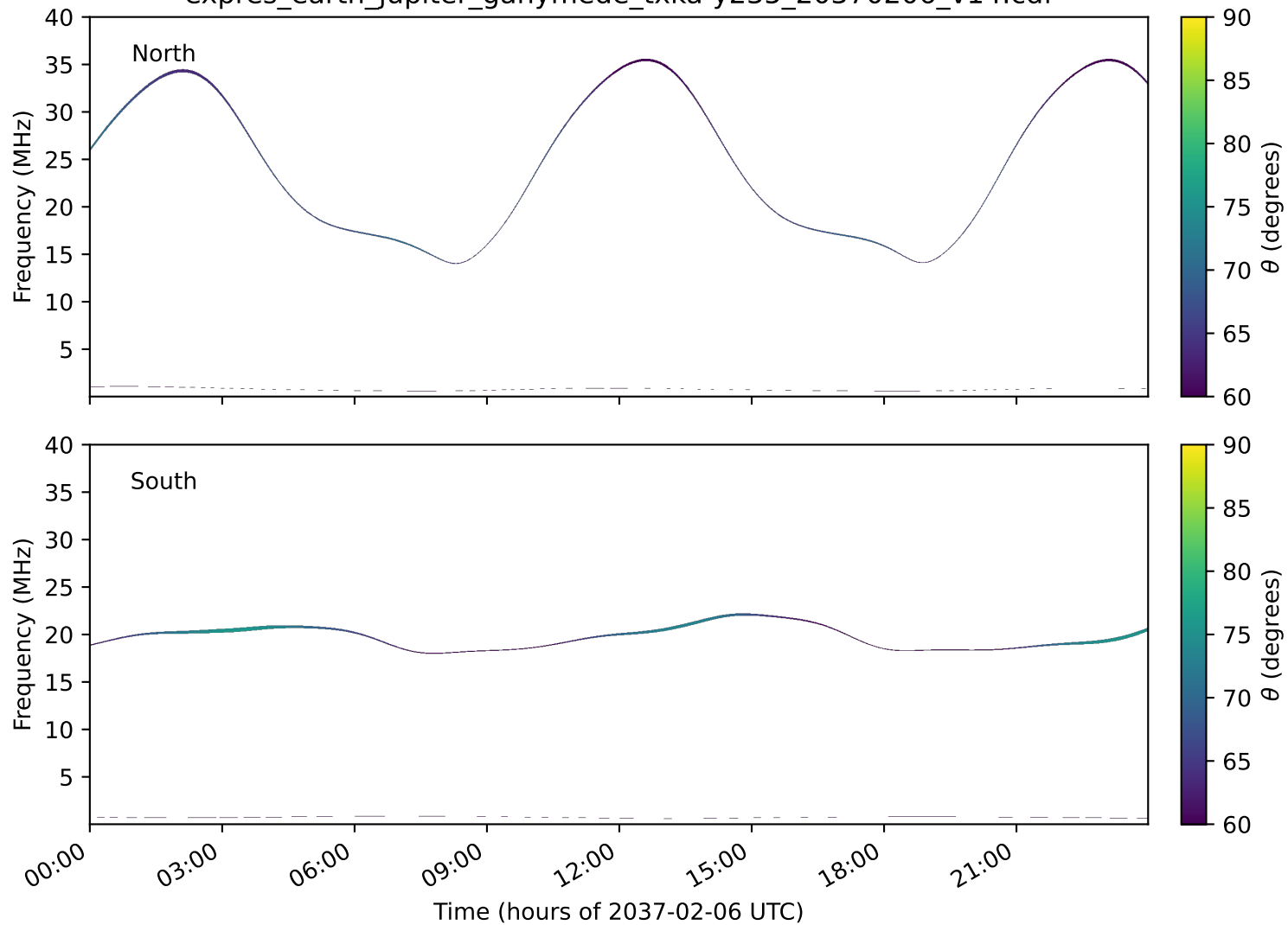
expres_earth_jupiter_ganymede_txka-y235_20370206_v14.cdf
