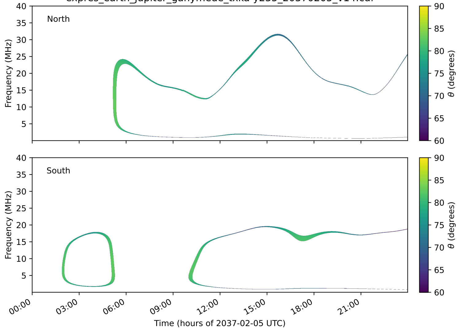
expres_earth_jupiter_ganymede_txka-y235_20370205_v14.cdf
