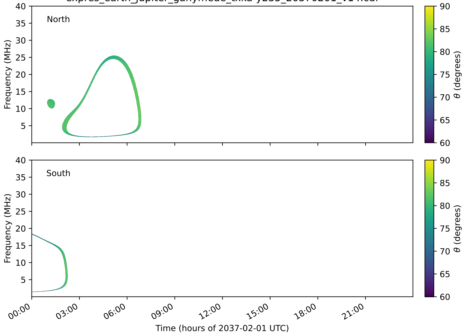
expres_earth_jupiter_ganymede_txka-y235_20370201_v14.cdf
